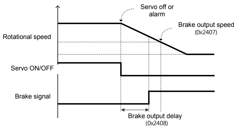
Timing diagram of signal output by brake output delay time (0x2408)
